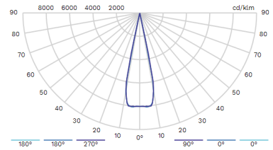
7050 Light Beam 25°
